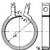
Figs. 2965-2966. Hose Clamp for 3 1/2-Inch Suction Hose.
